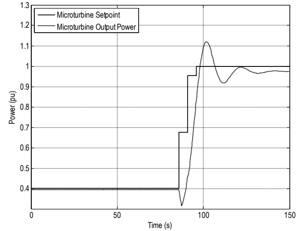
Fig. 9. Microturbine setpoint sequence.
