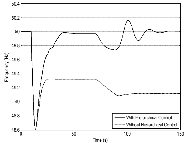
Fig. 6. Frequency deviation with and without hierarchical control.
