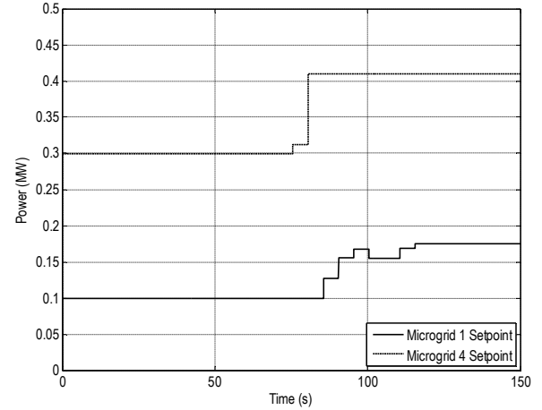
Fig. 8. Microgrid setpoints sent by the CAMC. Microgrid 4 is considered less expensive so its power setpoints increase first.
