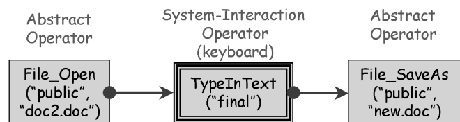
Fig. 5. A plan consisting of abstract operators and a GUI event.
