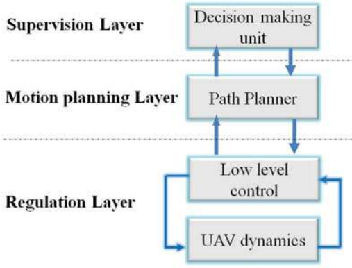
Figure 3. Hierarchical hybrid control structure of an autonomous UAV helicopter.
