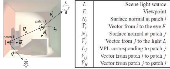
Figure 4: Notation used for image-space radiosity.
