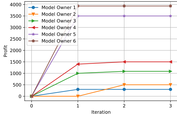
Fig. 8. Profit of each model owner for every iteration. Note that profit for iteration zero, i.e., initialization, is not computed.
