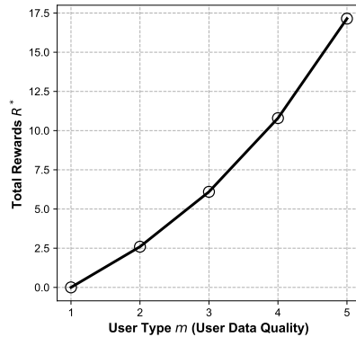
Fig. 3. Total rewards vs. User types.
