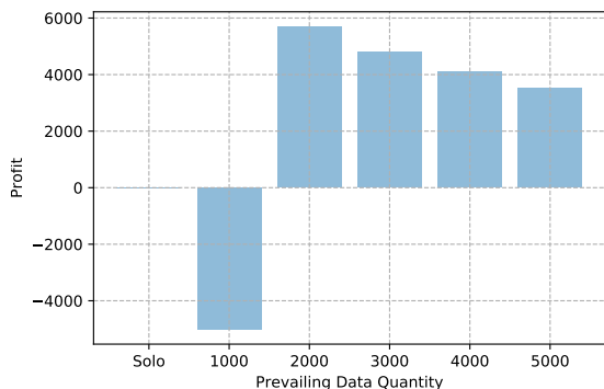
Fig. 5. Profit vs. prevailing data quantity.
