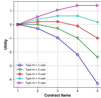
Fig. 4. User utility vs. contract items.
