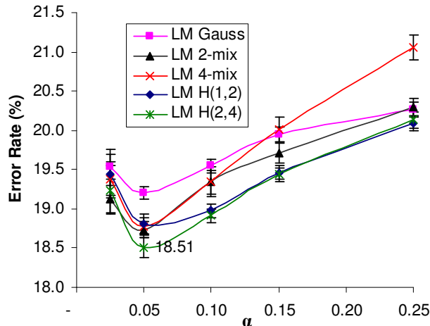
Fig. 2. Average error rate on the development set. Error bars show 0.25 standard deviation across feature sets.
