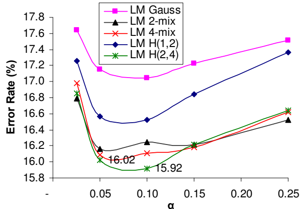
Fig. 3. Average error rate on the development set.
