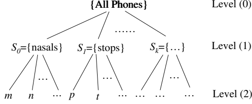
Fig. 1. Hierarchical classifier
