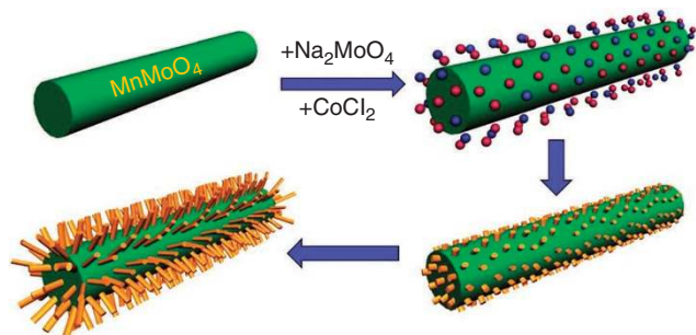
Figure 3 | The construction of hierarchical MnMoO 4 /CoMoO 4 nanowires. The green rod represents the backbone MnMoO 4 nanowire, and orange rods the CoMoO 4 nanorods. Red and blue balls are different ions dispersed in the aqueous solution.
