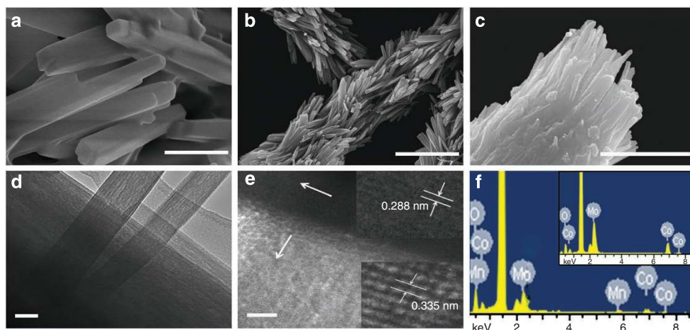
Figure 2 | Morphology characterization. (a) SEM image of the backbone MnMoO 4 nanowires. (b, c) SEM images of hierarchical MnMoO 4 /CoMoO 4 heterostructured nanowires. (d, e) TEM and high-resolution TEM images at the heterojunction of hierarchical MnMoO 4 /CoMoO 4 heterostructured nanowires. (f) The EDS microanalysis on selected areas. Scale bars, 1 μm (a–c); 20 nm (d); 5 nm (e).
