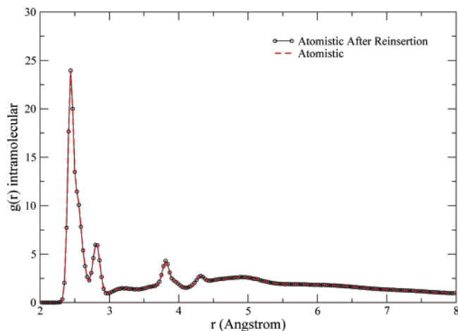
Figure 15. Intramolecular pair distribution function of PS chain from atomistic simulations and CG after reinsertion of atomistic detail (MW = 1 kDa, T = 463 K).
