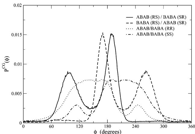
Figure 6. Probability distribution of dihedral angles ABAB and BABA for the coarse-grained effective beads at T = 463 K.
