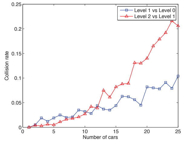
Fig. 4: Collision rates for level 1 and level 2 policies.
