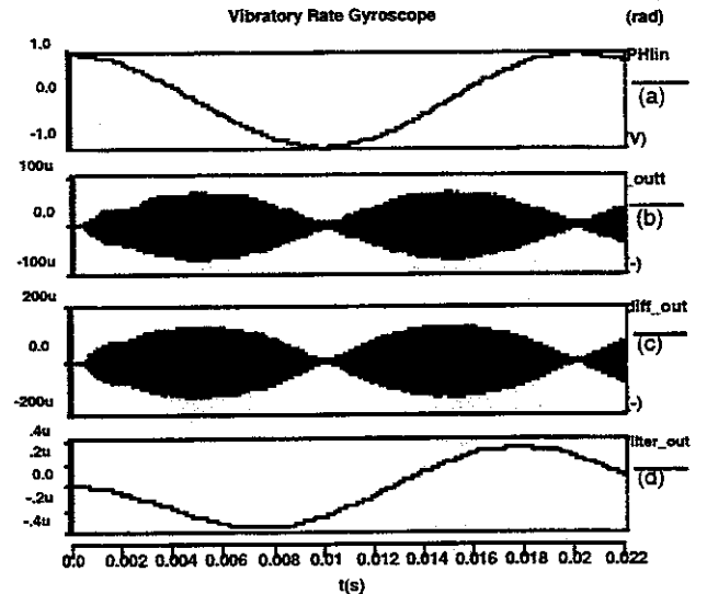
Figure 9. X-axis motion of the gyroscope caused from the input drive voltage ( v_{drive} ).
