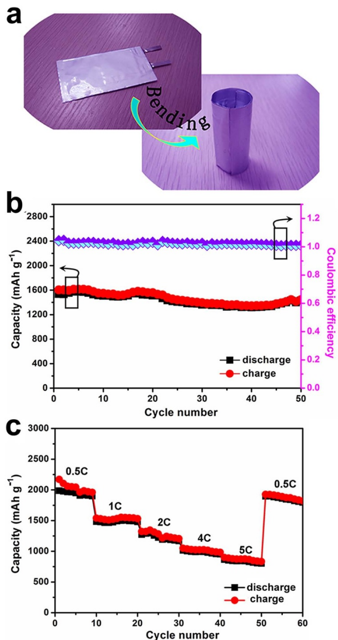
Figure 4 | Electrochemical properties of Si-based full batteries.
