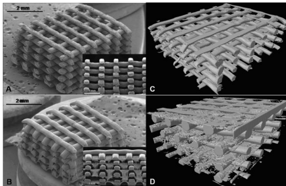
Figure 1. SEM and \mu -CT micrographs of the starch-based rapid prototyped, 6RP (A, C) and hierarchical fibrous scaffolds, 6RP + 5NFM (B, D)
