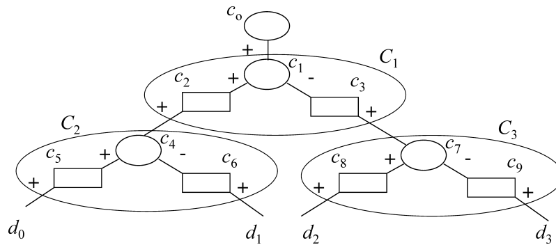
Fig. 2. An one-dimensional Haar + tree.
