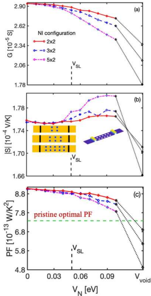
Fig. 9. Conductance G , Seebeck coefficient S , and power factor PF, for SL structures with barrier nano-inclusions (NIs) as shown in the inset of (b). Results for increasing NI barrier heights V_N are presented under electron-acoustic phonon-limited conditions. In (c), the PF of the optimized pristine channel is shown by the green dashed line. The red, blue and magenta lines show results in which the number of NIs increases from 2 \times 2 to 3 \times 2 and 5 \times 2 NIs, respectively—as shown in the inset of (b). The dotted black lines extend the results to the case where the NIs are replaced with voids, as shown in the inset of (b) as well. The SL barrier height, V_{SL} , is denoted as well. Reprinted from reference [71] with permission from APS (This figure is subject to copyright protection and is not covered by a Creative Commons license.).
