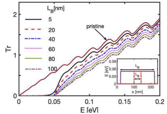
Fig. 5. Indication of the degree of relaxation of carriers on the barrier material as they propagate over it. The figure shows the NEGF calculated energy resolved transmission function Tr of the carriers in a channel with a single potential barrier with length L_B as indicated in the inset. Electron scattering with acoustic phonons only are considered in the calculation. Cases for different barrier lengths are shown from a large L_B = 100 nm taking over most of the channel (purple-dashed line), to a pristine channel (brown line). The ‘jump’ of the Tr from that of the larger barrier to that of the pristine material would indicate that carriers are more thermionically emitted over the barrier rather than ‘relaxing on it’ as the barrier length is scaled. Adopted from reference [81].
