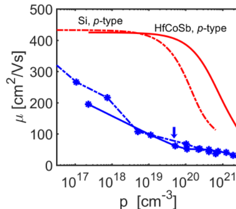
Fig. 10. The mobility of p -type Si (dashed lines) and the HfCoSb half Heusler alloy (solid lines), which is a promising thermoelectric material. The red lines indicate the phonon-limited mobilities, whereas the blue lines the phonon plus ionized impurity scattering limited mobilities.
