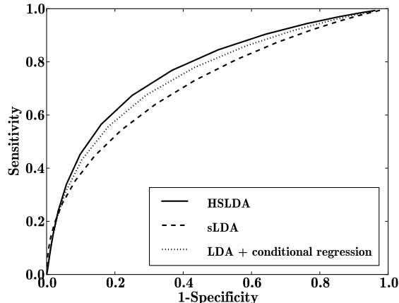
Figure 3: ROC curve for out-of-sample ICD-9 code prediction varying auxiliary variable threshold. \mu = -1.0 for all three models in this figure.
