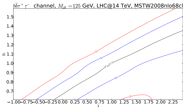
Figure 9. The 1\sigma and 2\sigma confidence regions in the y_t - \lambda plane at 600\text{fb}^{-1} for the b\bar{b}\tau^+\tau^- decay mode, derived using C_{HH} , within the SM ( \lambda_{\text{true}} = 1 and y_{t,\text{true}} = 1 ).
