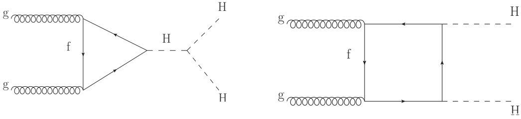
Figure 1. The Higgs pair production diagrams contributing to the gluon fusion process at LO are shown, for a generic fermion f .
