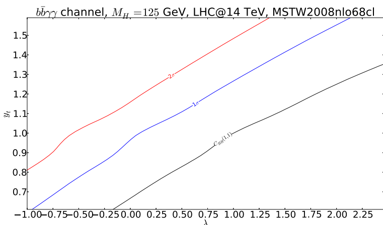
Figure 11. The 1\sigma and 2\sigma confidence regions in the y_t - \lambda plane at 600\text{ fb}^{-1} for the b\bar{b}\gamma\gamma decay mode, derived using C_{HH} , within the SM ( \lambda_{\text{true}} = 1 and y_{t,\text{true}} = 1 ). In the lower-right corner the exclusion is very weak and hence the one and two standard deviation curves are off the scale of the figure.
