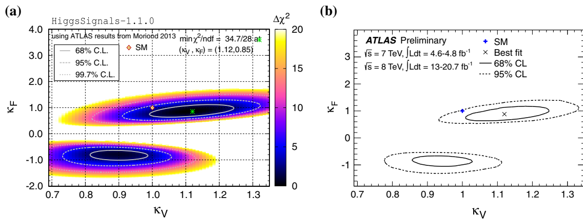
Fig. 7 Comparison of the two-parameter fits probing different coupling strength scale factors for fermions, \kappa_F , and vector bosons, \kappa_V , derived by HiggsSignals (a) and ATLAS [104] (b). The signal
