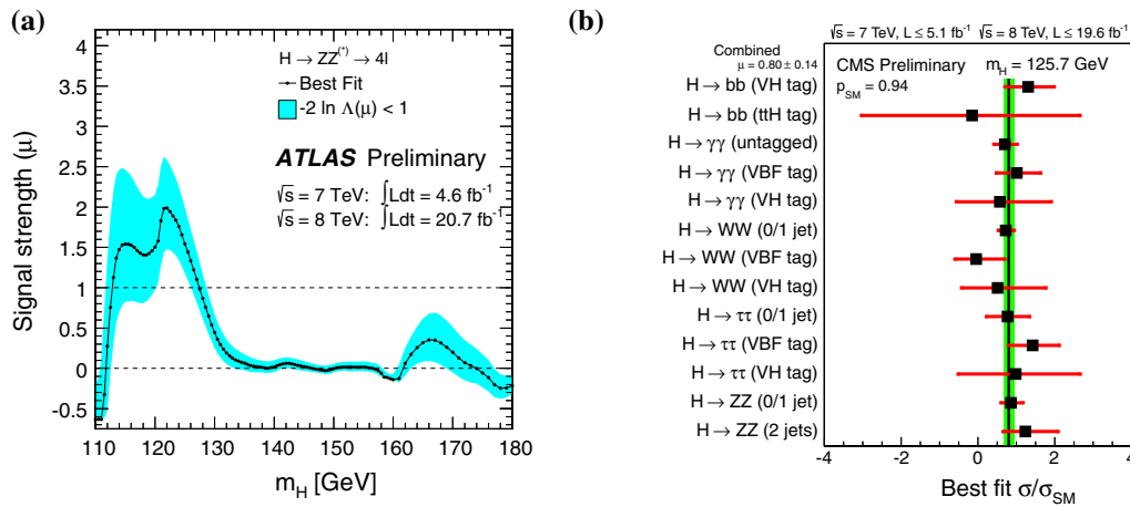
Fig. 1 Measured signal strength modifiers by ATLAS in the search for H \rightarrow ZZ^{(*)} \rightarrow 4l [75] (a) and the best fit rates (in all currently investigated Higgs decay channels) for a Higgs signal at m_H = 125.7 \text{ GeV} according to CMS [77] (b). a The best-fit signal strength \hat{\mu} for the LHC Higgs process (pp) \rightarrow H \rightarrow ZZ^{(*)} \rightarrow 4l , given as a function of the
