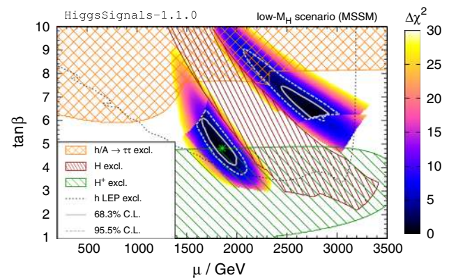
Fig. 14 \Delta\chi^2 distribution (HiggsSignals and HiggsBounds LEP exclusion \chi^2 added) in the low- M_H benchmark scenario of the MSSM [126]. The excluded regions and contour lines have the same meaning as in Fig. 12, except the red, finely striped region, which gives the 95 % C.L. exclusion from the CMS Higgs search H \rightarrow ZZ^{(*)} \rightarrow 4\ell [82], applied to the SM-like heavy \mathcal{CP} even Higgs boson. The best-fit point (indicated by a green star) is found at (\mu, \tan\beta) = (1850 \text{ GeV}, 4.9) with \chi^2/\text{ndf} = 80.3/66
