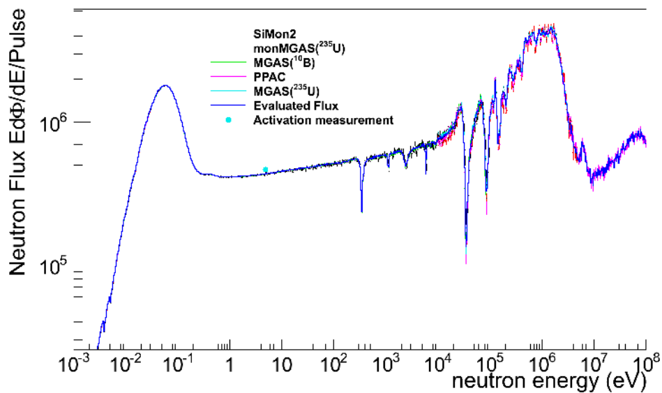
Fig. 8. Results from all measurements performed for the neutron flux determination and considered in the present analysis. The thick blue line corresponds to the evaluated flux. Each result has been normalized close to the thermal point to the value provided by SiMon2 measurement, while the cyan dot represents the integral measurement from the flux-averaged activation measurement.
