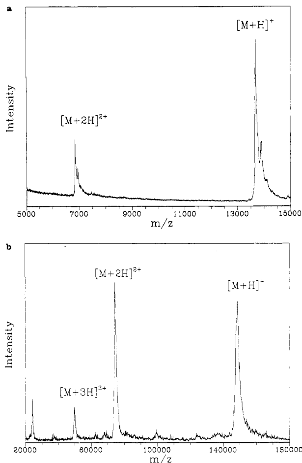
Figure 2. Mass spectra of two protein samples containing high contaminant concentrations: (a) bovine pancreatic ribonuclease A ( 5 \mu\text{M} protein solution in 1 \text{ M} urea); and (b) monoclonal immunoglobulin G, ( Mus musculus ) ( 5 \mu\text{M} protein solution in 50 \text{ mM} Tris HCl, \text{pH} = 7.4 ). Figure 1a is displayed in 20 \text{ ns} time bins and Figure 2b is displayed in 50\text{-ns} time bins. In both cases, horse skeletal muscle myoglobin was used as a calibrant for molecular mass determination.
