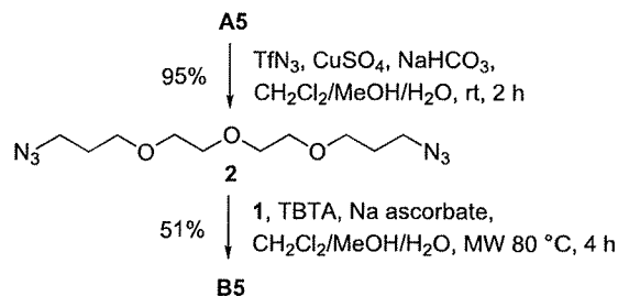
Scheme 1: Synthesis of glycocluster B5 with isolation of the intermediate diazide 2 .
