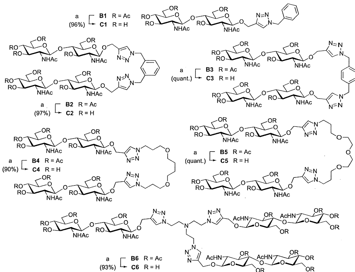
Scheme 2: Deacetylation of glycoconjugates B1–B6 . (a) NaOMe, MeOH.
