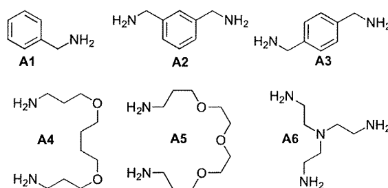
Figure 1: Amines used for the synthesis of glycoclusters.
