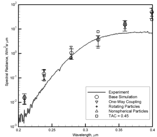
Fig. 12 UV spectral radiance at the onboard sensor.
