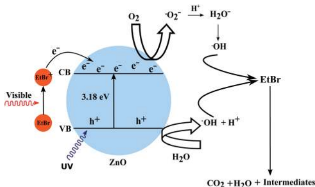
Fig. 17 The proposed mechanism to explain the photocatalytic degradation of EtBr.
