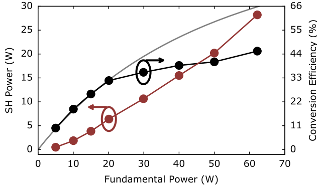
Fig. 2. Generated second-harmonic (SH) average power at 780 nm (red points) and SHG conversion efficiency (black points) as a function of fundamental (1560 nm) average power, connecting lines are a guide for the eye. The SHG conversion efficiency is fitted with a \tanh^2 curve, according to Eqn. 1 (grey line).
