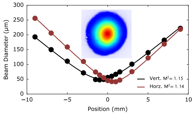
Fig. 4. Beam diameter (points) of the generated 780 nm at full power through the focus of an f=120 mm lens in the horizontal and vertical axes with Gaussian beam caustic fits (lines). Inset: typical CCD image of the collimated beam profile.
