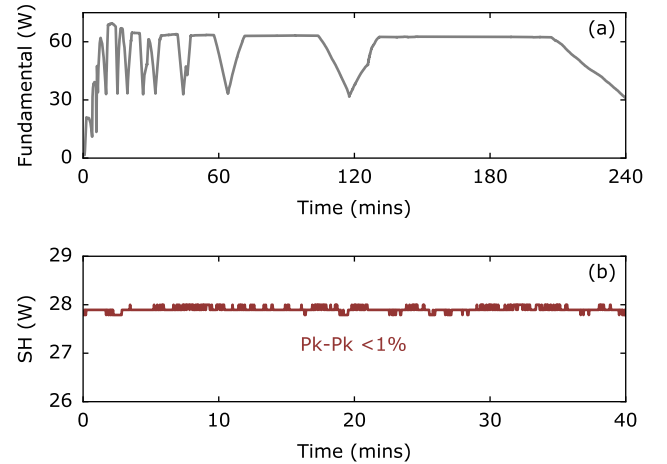
Fig. 3. (a) Polarized fundamental power as a function of time from turn-on, demonstrating oscillations in the degree of polarization. (b) Power stability of the second-harmonic (SH) over a 40 minute period without adjustment of the fundamental polarization.
