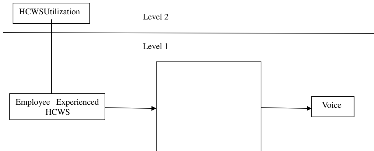
FIGURE 1 Theoretical Model
