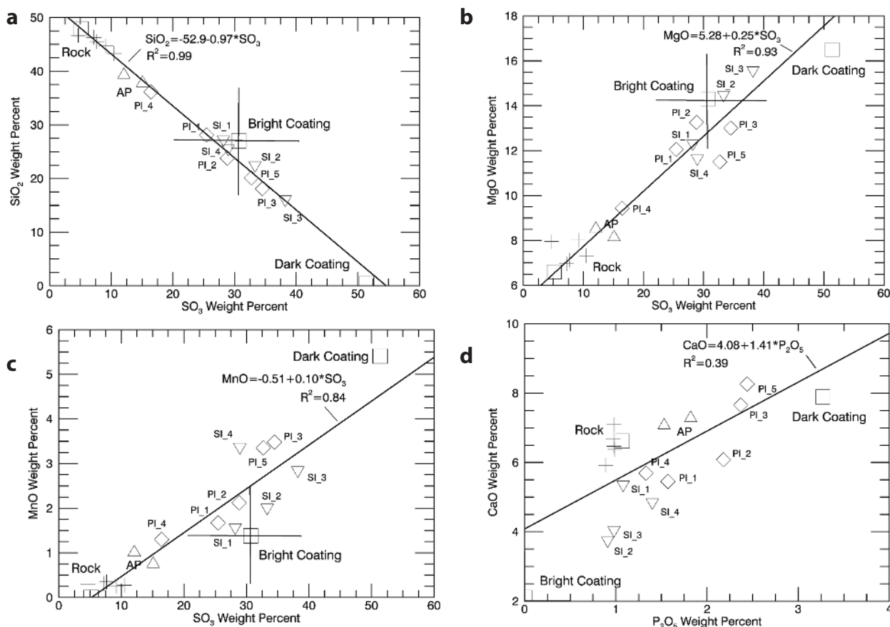
FIGURE 21. Bivariate plots are shown of \text{SiO}_2 , \text{MgO} , and \text{MnO} as a function of \text{SO}_3 contents, along with \text{CaO} as a function of \text{P}_2\text{O}_5 , for Cook Haven APXS measurements. Bright and dark coatings and rock retrieved end-member compositions are also shown. Error bars are plotted for the bright coating (Table 2). For the other two end-members the errors are comparable to the box symbol sizes. Least-squares linear fits to the APXS data (not end-members) are shown as straight lines, along with the square of the Pearson linear correlation coefficient. These bivariate plots were chosen to illustrate trends with high correlation coefficients, based on results from the correspondence analysis shown in Figure 20.
