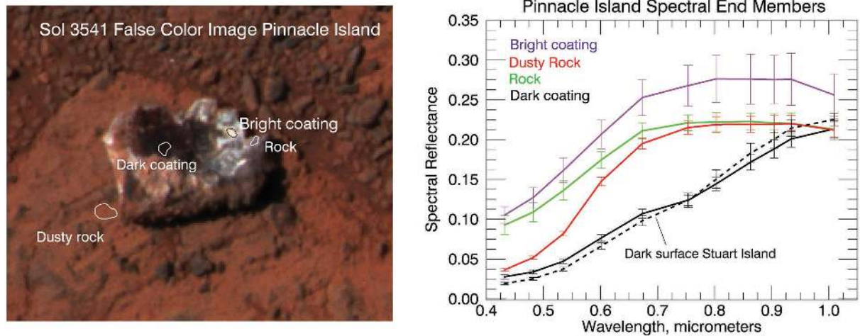
FIGURE 18. Locations of Pancam spectral end-members derived from the unmixing algorithm are shown on the Pancam false color image on the left, and mean spectra for these regions are shown on the right. Also shown is the mean spectrum for the dark area on Stuart Island. One standard deviation error bars are also plotted. The dark coating spectra for the Island rocks are indistinguishable and unique for any Pancam observation. The spectra lack the ferric absorption edge shortward of \sim 0.7 \mu\text{m} that is characteristic of martian spectra, and evident for the other three spectra shown in the figure. The dusty rock spectrum has the deepest ferric absorption edge, followed by the bright coating spectrum, and the rock spectrum has the shallowest absorption.
