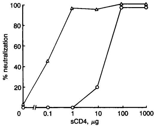
FIG. 5. Neutralization of the primary isolate HIV-1AC after a single passage in PBMCs (○) and after propagation in H9 cells for approximately 1 year (△).
