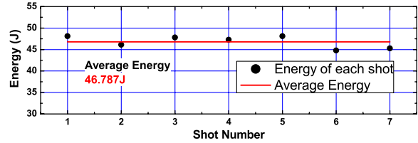
Fig. 2. (Color online) Measured output energies for 105 J pump energy in the booster amplifier. For the seven-shot measurements, the maximum energy was 48.1 J and the minimum energy was 44.8 J. The rms was about 1.5%.
