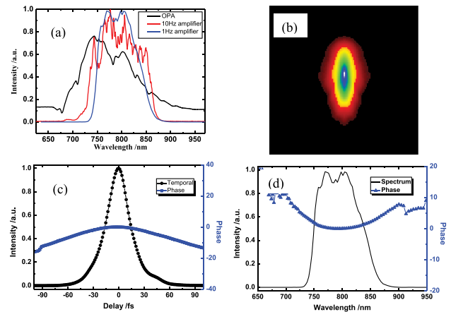
Fig. 3. (Color online) (a) Spectrum of each stage, (b) the trace of the FROG measurement, (c) the measured pulse duration, and (d) the spectrum of compressed pulse using the video FROG instrument.
