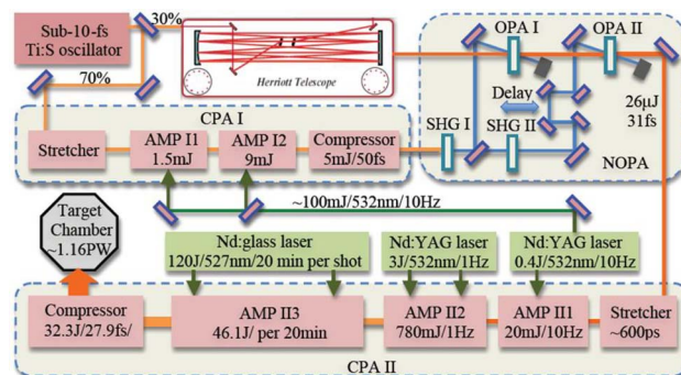
Fig. 1. (Color online) Schematic experimental setup of the DCPA.
