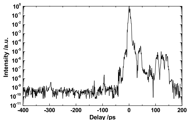
Fig. 4. Contrast ratio of the compressed pulse within the time scale from -400 to 200 ps.
