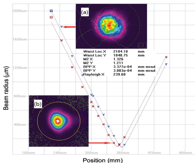
Fig. 5. (Color online) (a) Near-field and (b) far-field beam profiles and M^2 factor of the compressed pulse in the second CPA stage.
