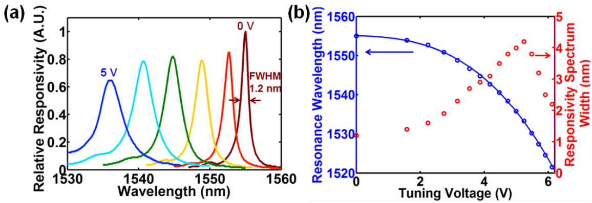
Figure 5.3 (a) Relative responsivity spectrum of an HCG detector versus tuning voltage. A minimum spectrum width (FWHM) of 1.2 nm is achieved at 0 V tuning voltage. (b) Resonance wavelength (blue) and responsivity spectrum width (red) versus tuning voltage. A 33.5 nm tuning range is achieved with a tuning voltage range of 6.1 V. The dots are experimental measured data, and the blue curve is a parabolic fitted curve for the resonance wavelength and tuning voltage. The non-uniformity in the responsivity spectrum width is due to the deformation of the HCG mirror when being actuated, and can be much improved with an optimization of the MEMS design for the HCG.
