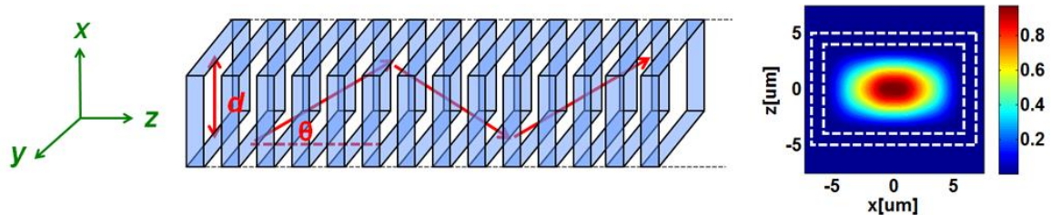
Figure 3.18 Schematics of a 3D cage-like HCG HCW and the mode profile of the fundamental mode. The color code indicates the normalized electrical field intensity.
