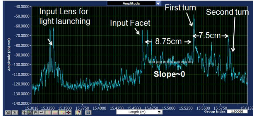
Figure 3.17 Loss measurement through optical backscatter reflectometer on an HCG-DBR hybrid HCW. The spikes indicate large reflections, typically because of the interfaces between different optics in the optical path. The slope of the signal indicates propagation loss. The average slope is around zero for the first 8.75 cm straight waveguide, indicating an extremely low loss. After the first turning however, the slope becomes signification, indicating a high loss. This is due to the fundamental mode scattering into high order modes, which have much higher propagation losses. The noise is due to environmental vibration and defects along the waveguide.
