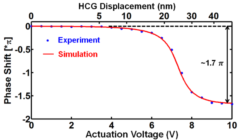
Figure 4.14 Reflection phase shift versus applied voltage on a single HCG-APF of the phased array. \sim 1.7\pi phase shift is achieved within 10V actuation voltage range at a wavelength of 1556 nm; this corresponds to a displacement of \sim 50 nm of the HCG. This APF design enables a small actuation distance for a large phase change. The experimental data (blue dots) are fitted with the simulation results with the DBR and HCG reflectivity of 0.9977 and 0.935 respectively (red curve).
