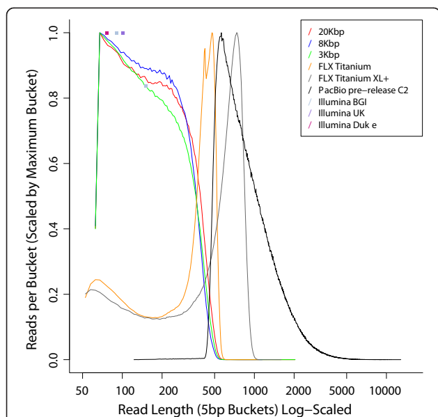
Figure 1 The distribution of read lengths in 454, Illumina and PacBio budgerigar sequences. The reads are binned into 5 bp buckets based on their lengths, and the fraction of reads (normalized by the size of the largest bucket) falling into each bucket is shown. Thus, curves shifted towards the right indicate longer read lengths. The reads labeled “20 Kbp”, “8 Kbp” and “3 Kbp”, “FLX Titanium” and “FLX Titanium XL+” are 454 reads. The reads labeled “PacBio pre-release C2” are uncorrected PacBio reads. The Illumina read lengths appear as colored square boxes, since these read lengths are uniform. The “Illumina Duke” reads are of length 76, The “Illumina UK” reads are of length 101, and the “Illumina BGI” reads are of lengths 90 or 150. The longest reads come from PacBio sequencing, followed by 454 FLX + (i.e., FLX Titanium XL+) sequencing.
