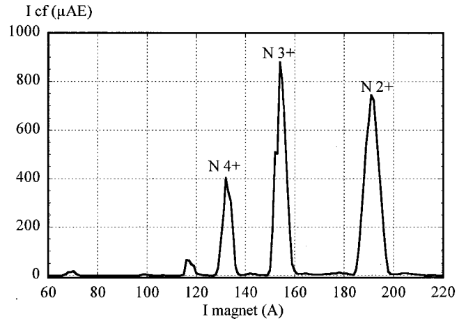
FIG. 3. N 3+ up to 900 μA with ∅ 2 mm extraction hole at 48 kV.
