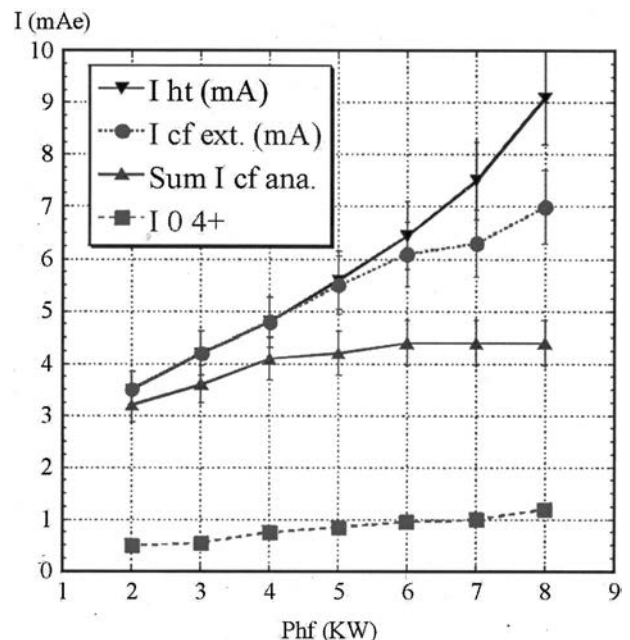
FIG. 4. Power dependence of the drain current ( I_{ht} ), the Faraday cup current at the exit of the puller ( I_{cf ext.} ) and the total current of the spectrum at the exit of the bending magnet ( \sum I_{cf ana.} ).
