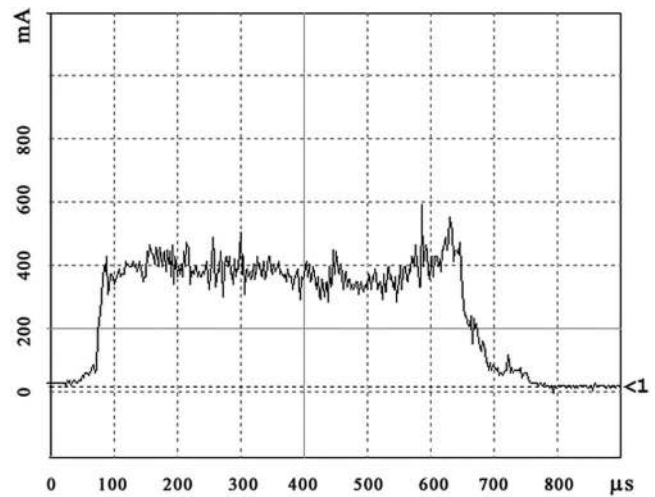
FIG. 4. Example of Faraday cup current waveform.
