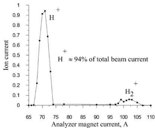
FIG. 6. Mass-analyzed ion beam spectrum normalized to the total beam current.
