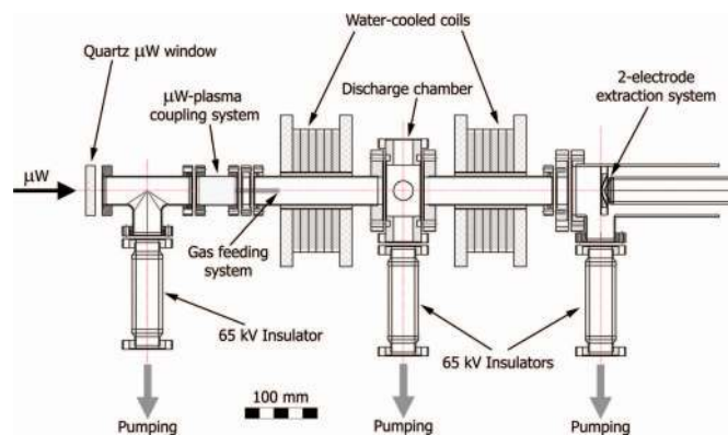
FIG. 1. SMIS 37 experimental setup.
