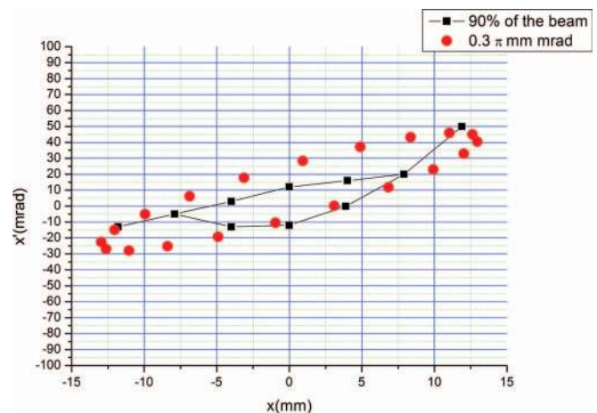
FIG. 5. An example of the phase space distribution of the 450 mA beam.
