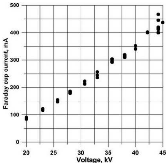
FIG. 3. Faraday cup current versus extraction voltage.
