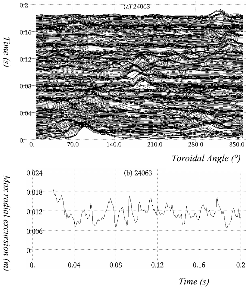
Fig 1. Radial displacement (a.u.) of the last closed magnetic surface due to m=1 modes in shot 24063 as a function of the toroidal angle and of time (vertical direction). b) Absolute maximum radial displacement (m) of the plasma as a function of time.
