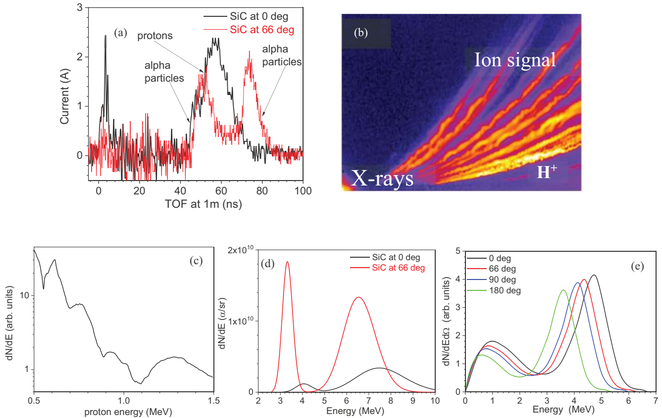
FIG. 3. (a) TOF spectra from detectors placed at 0^\circ (black curve) and 66^\circ (red curve) normalized at 1 m distance. (b) Raw data from TP spectrometer, showing the different ion species deflected from the electric and magnetic field of the detector. (c) Proton energy distribution from the TP evaluation. The measured data have been smoothed, in the black line, to better understand the behavior of the distribution. (d) \alpha -particle energy distribution from TOF deconvolutions at 0^\circ (black curve) and 66^\circ (red curve). (e) Theoretical spectra in the reaction channel via {}^8\text{Be}^* , for different values of the detection angle \theta . Calculations refer to a 675 keV proton impinging on {}^{11}\text{B} at rest along \theta = 0 (after Stave et al. [4]).
