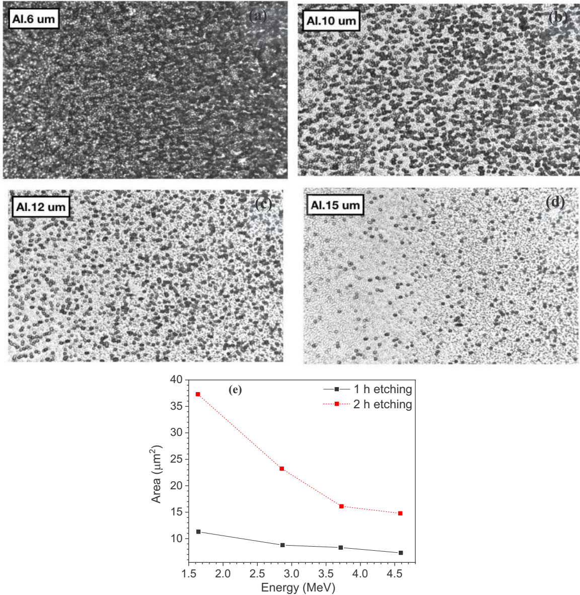
FIG. 4. Images from CR39 nuclear track detectors placed at 66^\circ , covered with 6 \mu\text{m} (a), 10 \mu\text{m} (b), 12 \mu\text{m} (c), and 15 \mu\text{m} (d) Al filter, obtained after 1 h of etching time. (e) Evolution of the \alpha -particles tracks as a function of the incident energy. The exposed CR39 were etched in a 6.05N NaOH solution at a constant temperature of 80^\circ\text{C} . Different curves in the plot represent two different etching times: 1 h (black curve) and 2 h (red curve).
