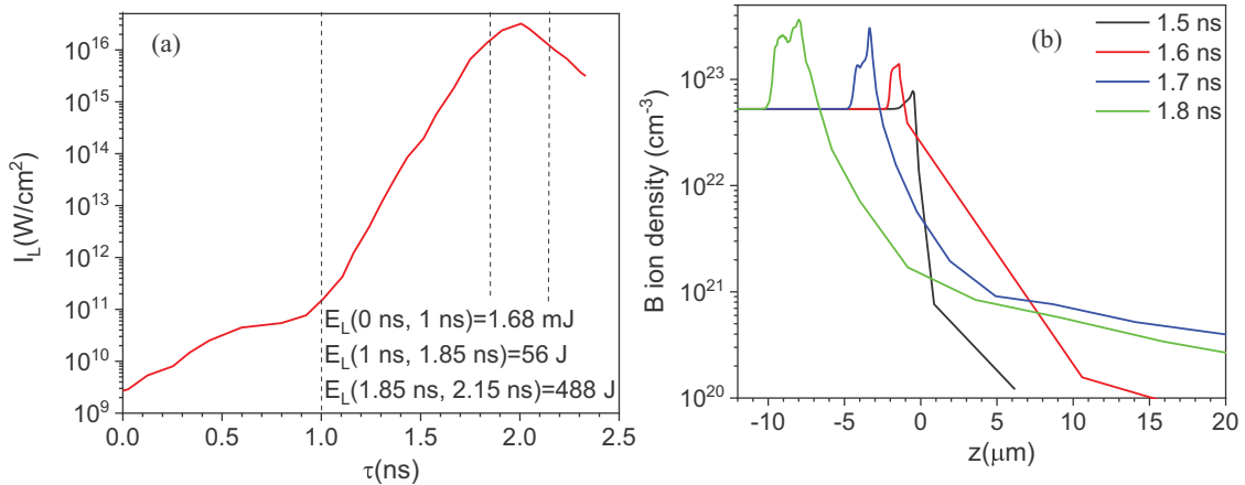
FIG. 6. (a) Temporal profile of the laser intensity on the target (measured). The laser energy contained in the time window up to 1.85 ns represents the prepulse of the laser. (b) PALE hydrodynamic simulation of the B ion density profile at different times from the start of the laser action ( t = 0 ). Profiles are taken at the origin of the transverse coordinate (center of the laser spot). At t = 0 , the longitudinal coordinate, z , is defined as follows: z = 0 is the target surface, z > 0 is a vacuum, and z < 0 is the target bulk.
