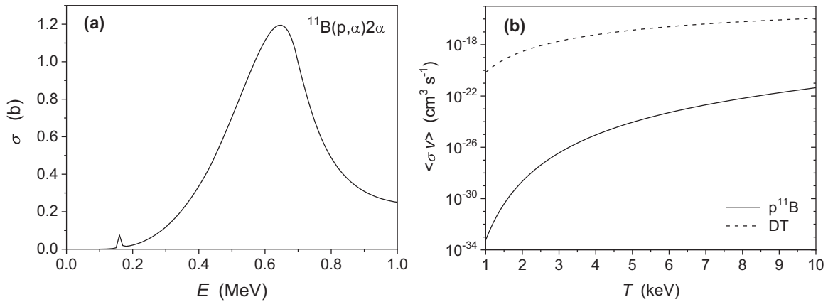
FIG. 1. (a) p\text{-}^{11}\text{B} fusion cross section as a function of proton energy in the lab, based on the analytic approximation of Nevins and Swain [2]. (b) Low-temperature reactivity for pB fusion and, as a term of comparison, DT fusion. Plots are based on the analytic approximations of Refs. [2] and [25], respectively.
