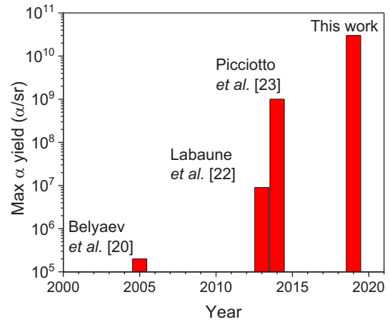
FIG. 9. Progression of the most important experimental achievements reported in the literature in terms of maximum \alpha particles/sr.
