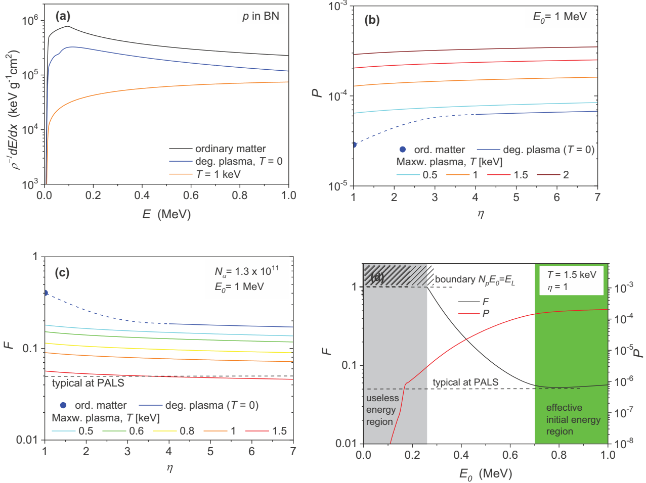
FIG. 7. (a) Electronic mass stopping power for protons in BN as a function of projectile energy, for ordinary bulk, fully degenerate plasma, and high-temperature plasma, respectively. Stopping powers are calculated at the density \rho_0 . (b) Fusion probability for 1 MeV protons as a function of bulk compression, for values of interest of the temperature. The dashed curve represents intermediate ionization states between ordinary matter and degenerate plasma, and is drawn for eye guidance only. (c) Fraction of proton-to-laser energy needed to produce the given number of \alpha particles, plotted as a function of bulk compression, for values of interest of the temperature. (d) Proton-to-laser energy fraction required for N_\alpha = 1.3 \times 10^{11} as a function of the initial proton energy (black curve), in a bulk at T = 1.5 keV, \eta = 1 . The relating fusion probability P(E_0) is also shown (red curve).
