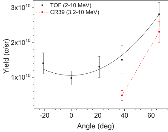
FIG. 5. Angular distribution obtained from TOF measurements (in black) compared with results obtained from CR39 (in red).
