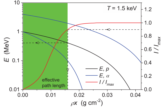
FIG. 8. Energy vs path-length curves for protons and \alpha particles in a BN bulk at T = 1.5 keV. Initial energies are 1 MeV for protons; 1 MeV and 4 MeV for \alpha particles, respectively. The normalized fusion probability up to a distance \rho x , I(\rho x)/I_{\max} , is also shown during proton slowing down. Its wide plateau limits the thickness of the bulk region, which is needed for \alpha production (dashed-line construction). Both groups of \alpha particles have enough kinetic energy to leave that region.
