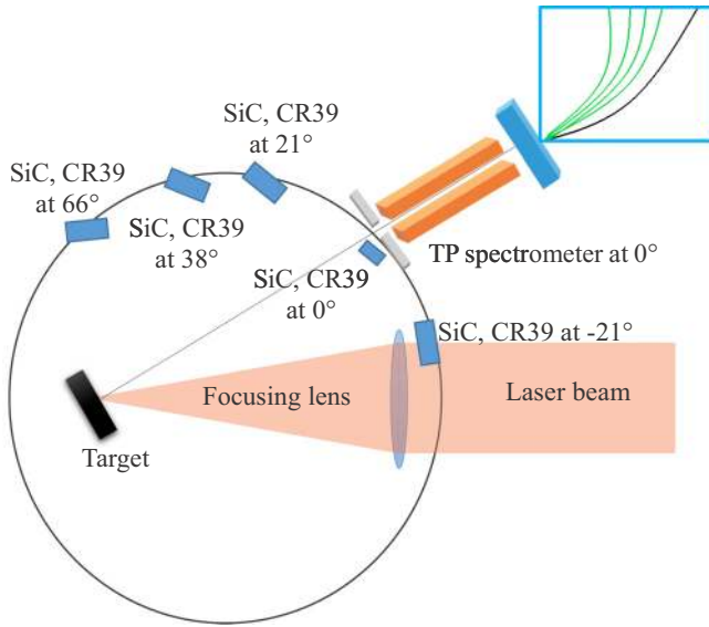
FIG. 2. Experimental setup used during this experimental campaign. The laser beam passing through a focusing lens reaches a final dimension of 80 \mu\text{m} onto the target ( 30^\circ incidence angle). Particle emission is mainly along the normal to the target surface. Several detectors (SiC and CR39) were placed at different angles. A Thomson Parabola spectrometer (TP) was placed at 0^\circ .
