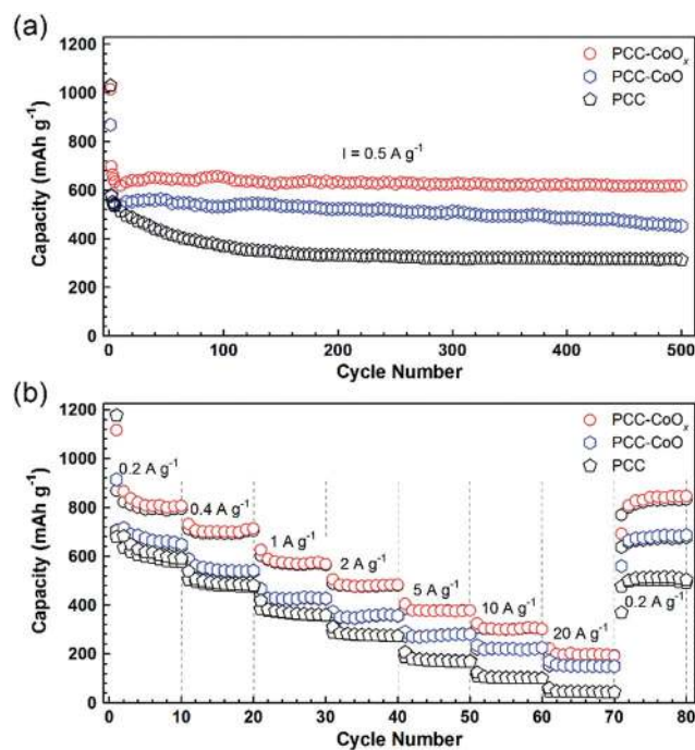
Fig. 4 (a) Cycling behaviours of the PCC–CoO x , PCC–CoO, and PCC electrodes at the same current density of 0.5 \text{ A g}^{-1} . (b) Rate performances of the PCC–CoO x , PCC–CoO, and PCC electrodes at various current densities ranging from 0.2 to 20 \text{ A g}^{-1} .
