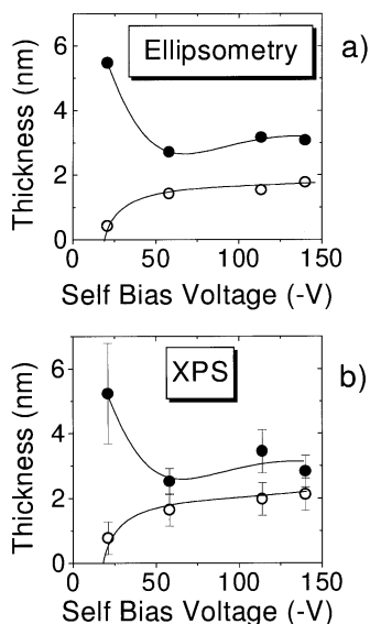
FIG. 7. CF x and SiF y layer thicknesses determined by (a) ellipsometry and (b) XPS. The samples analyzed were processed in a 40 sccm CHF 3 discharge at 6 mTorr and maintained by 600 W inductive power.
