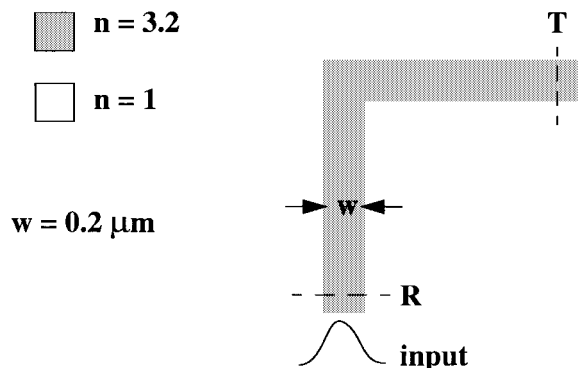
Fig. 1. Schematic of a 90^\circ sharp waveguide bend made of a high index waveguide n = 3.2 surrounded by air. The cross sections where transmission and reflection are calculated are also shown.
