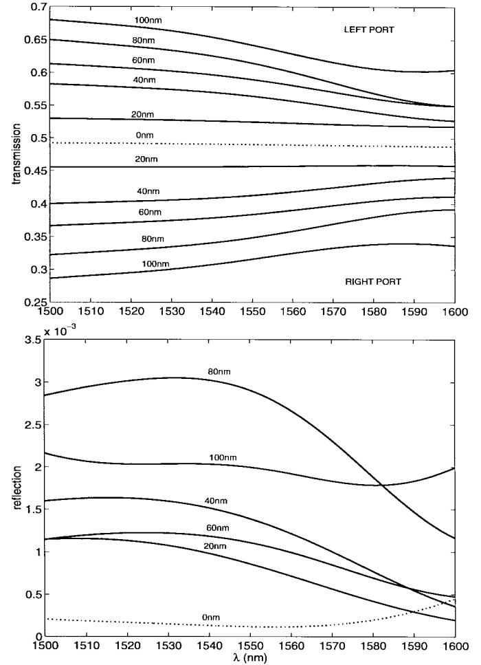
Fig. 16. Power distribution and reflection at the ports of an asymmetric T-junction for displacement of the input waveguide in the range from 0 to 100 nm.
