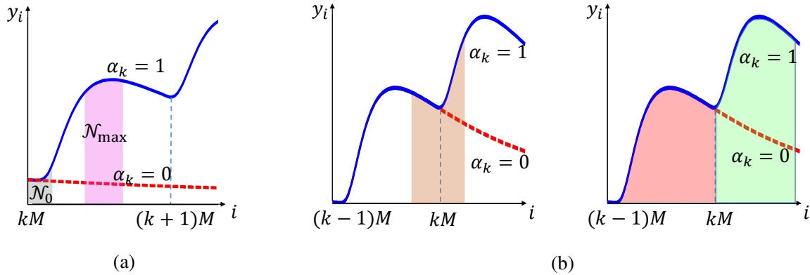
Fig. 2. Illustration of sub-metrics. (a) gives the local rising edge metric z_{k,1} , whilst (b) shows the successive properties that contains the inflexion metric z_{k,2} and the energy-difference z_{k,3}
