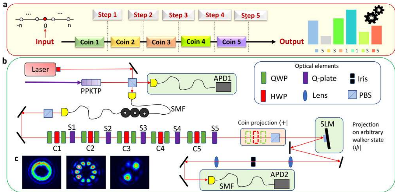
Figure 2. Setup of the arbitrary qudits generation through quantum walks. a) Schematic of the protocol: at each step, the coin operator is changed to have the desired walker state at the output. b) Experimental setup: A ppKTP source generates pairs of photons, which are then coupled to SMF. One photon acts as a trigger, while the other one is prepared in the initial |\psi_0\rangle with a PBS and a polarization controller. Coin and shift operators are implemented with a set of wave plates and q -plates, respectively. The detection consists of a PBS, followed by an SLM, an SMF, and avalanche photodiode detectors (APD). c) Pictures of the OAM modes after the PBS for (from right to left) OAM eigenstate corresponding to \ell = 5 ; balanced superposition of \ell = \pm 5 ; balanced superposition of all OAM components involved in the quantum walk dynamics, that is, \ell = \pm 5, \pm 3, \pm 1 . Reproduced with permission. [115] Copyright 2019, American Physical Society.
