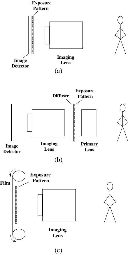
Figure 2: One way to achieve spatially varying pixel exposures is by using an optical mask with an array of cells with different transparencies. (a) Such a mask can be placed adjacent to the image detector array. (b) The mask can also be fixed at a distance from the detector by using a primary lens to focus scene rays onto the mask and an imaging lens to project radiance at the mask onto the detector plane. (c) For film cameras, the mask can be placed adjacent to the film area that is exposed to the scene.
