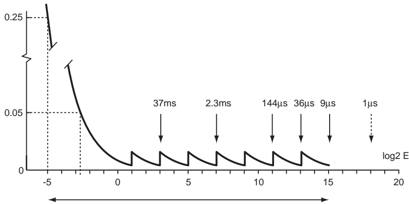
Figure 5: Relative quantization error for the example implementation (black, thick curve). The dynamic range of the demo image on page 1 is indicated at the bottom. The dynamic range of the capture can be extended further by making the shortest exposure 1 \mu s. More exposures could be added also at the low end of the scale, but that would require a lower frame rate than the current 25 frames per second. Also, while quantization is the dominant source of error for high intensities, low intensities are also affected by thermal noise, which limits the attainable image quality for longer exposures unless the sensor is cooled.
