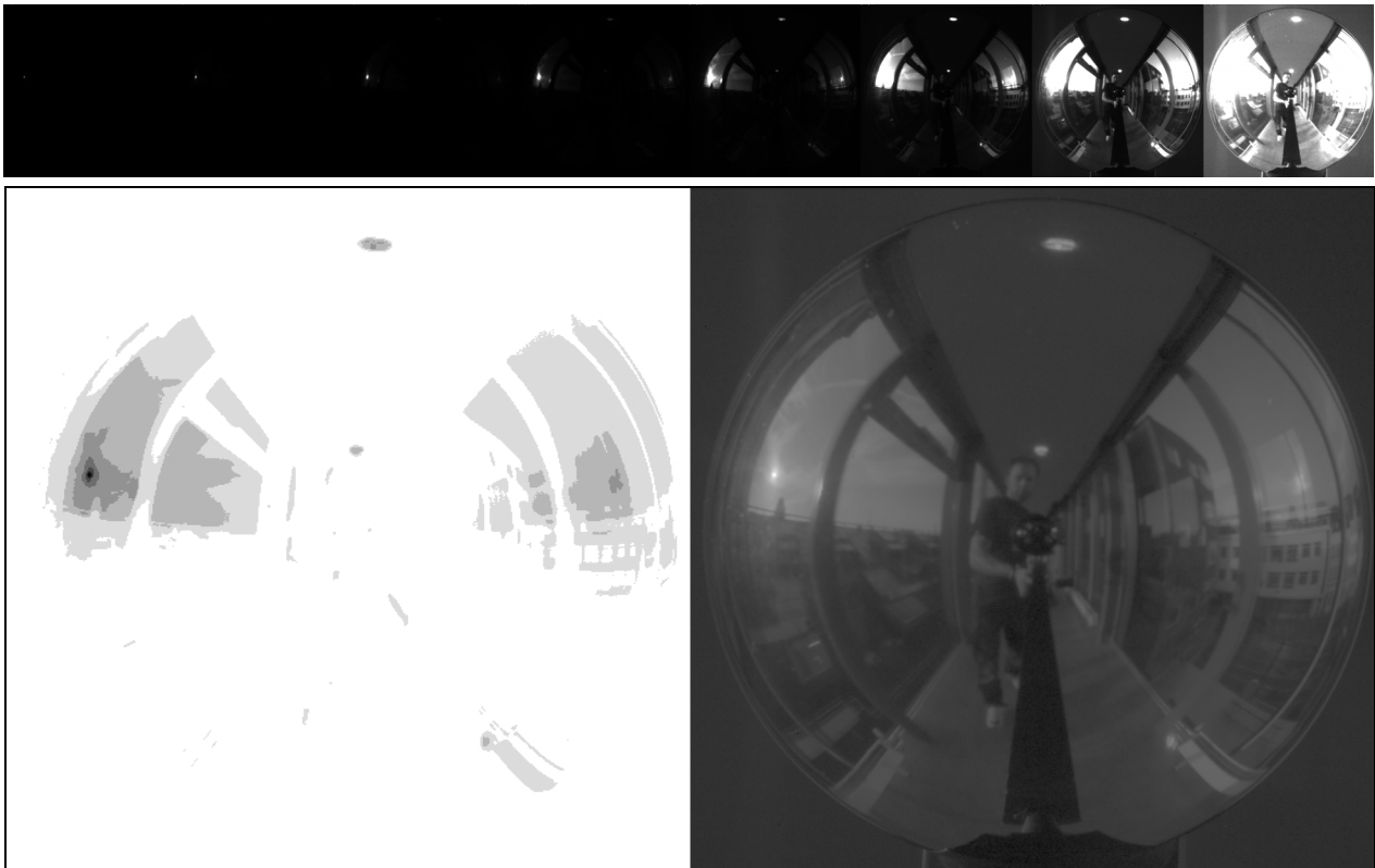
Figure 1: Sample image from a video stream from the system. Top: eight separate 8-bit linear exposures. Bottom left: index map showing which exposure was selected for each pixel in the final composited HDR image. Bottom right: log-mapped HDR image. The resolution is 512 \times 512 pixels, and the full HDR image was captured in 40 ms. The dynamic range of this image exceeds 1,000,000:1, and all pixels in the image have a valid photometric value.
