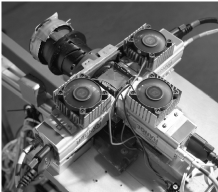
Figure 3: The single lens setup with an RGB beamsplitter (left), and the simpler setup with three separate lenses and RGB color filters pointing at a reflective sphere (right). Both use three separate, unmodified but reprogrammed C55 camera units.
