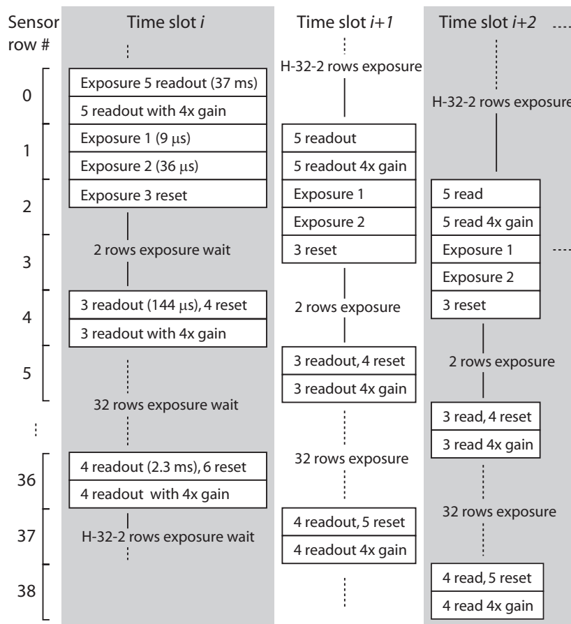
Figure 4: Diagram of the capture algorithm, somewhat simplified for presentation. The progressive image exposure and readout from a rolling shutter algorithm effectively removes any delay between subsequent exposures within each HDR frame. Each time slot is 78 \mu s, during which resets and readouts of several different sensor rows are performed. One full frame is captured in as many time slots as there are rows in the output image.
