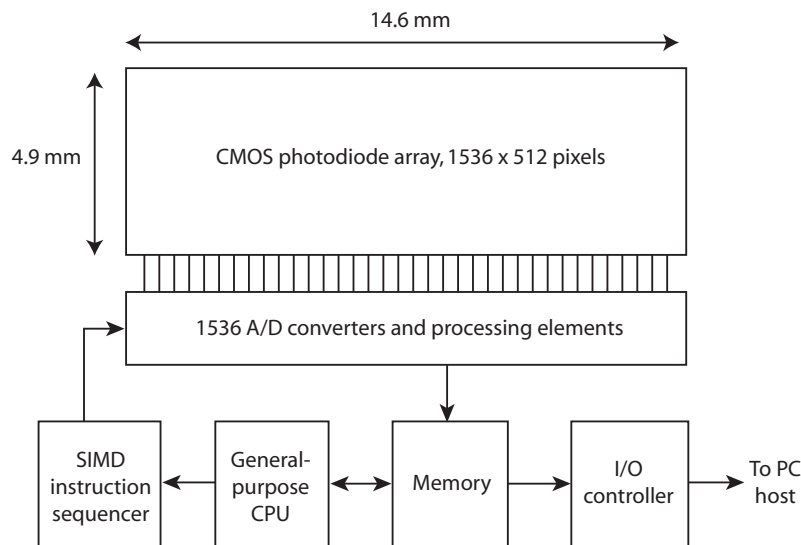
Figure 2: System overview of the Ranger C55 camera hardware (simplified)
