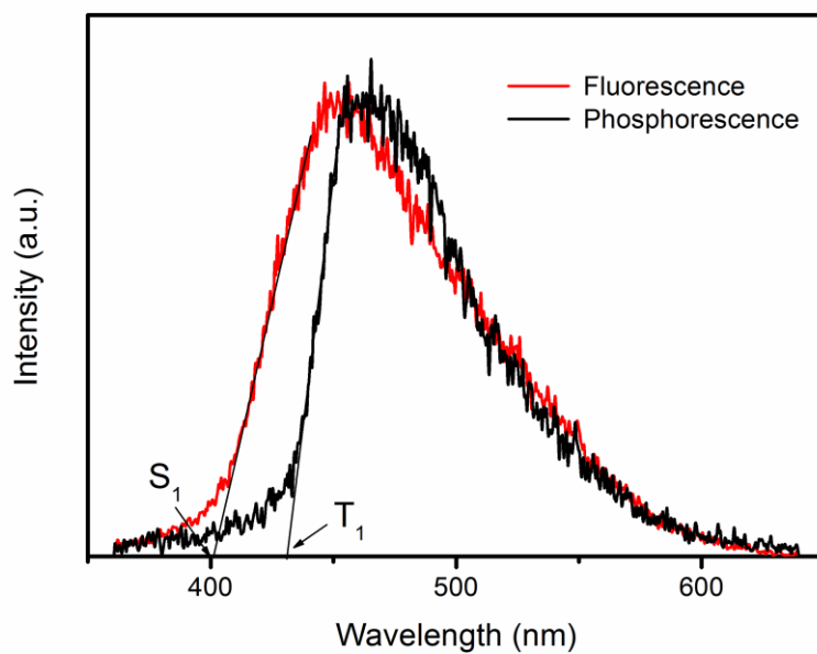
Fig. S2 Fluorescence (< 0.1 \mu s) and phosphorescence (> 0.1 \mu s) spectra of a DPEPO film doped with 10 wt% DMOC-DPS at 10 K.
