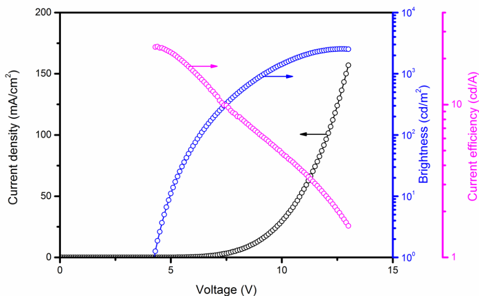
Fig. S3 Relationship between brightness, current density, and voltage for the OLED based on DMOC-DPS.
