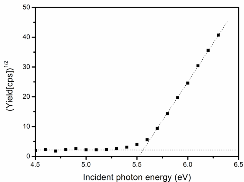
Fig. S1 The photoelectron yield spectrum of the neat film of DMOC-DPS. The HOMO level of DMOC-DPS is at 5.55 eV, in contrast to 5.81 eV for DTC-DPS. 1
