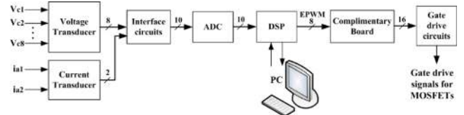
Fig. 23. 5-level single-phase-leg MMC signal process.
