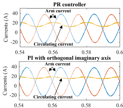
Fig. 25 Simulated arm and circulating currents with mismatched capacitance under PI and PR control.
