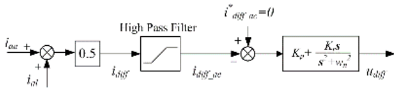
Fig. 14. PR control block for circulating current suppression.
