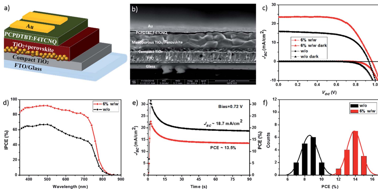
Fig. 3 (a) Schematic device structure of perovskite solar cell. (b) Cross-sectional SEM image of the device consisting of FTO-glass/compact \text{TiO}_2 /mesoporous \text{TiO}_2 /perovskite/PCPDTBT:F4TCNQ/Au. (c) J - V characteristics measured under AM 1.5 simulated sunlight ( 100 \text{ mW cm}^{-2} irradiance) and in the dark. (d) IPCE spectra of PSC devices based on PCPDTBT with and without doping F4TCNQ as HTMs. (e) Steady-state maximum photocurrent (black) and power output (red) measurement for a representative device based on PCPDTBT doped with 6% F4TCNQ as a HTM. (f) Histogram of power conversion efficiency comparison between PCPDTBT with and without F4TCNQ as HTM (15 cells for each group).
