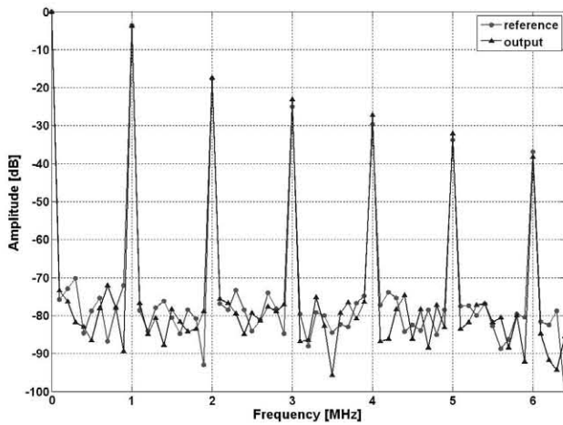
Figure 11. Spectrum of the reference and output signal when a rectified 500kHz sine wave is used as the reference. All the values are scaled to the dc value of the signal
