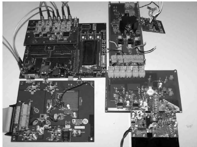
Figure 12. Photograph of the implemented EER Transmitter (on the right) with FPGA board, A/D and D/A converters (on the left)
