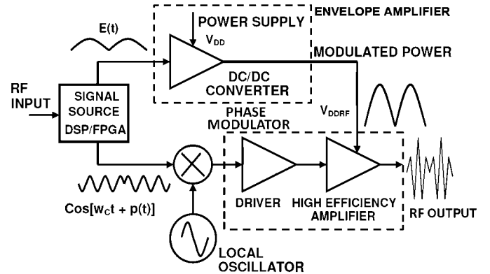
Figure 1. Block Scheme of Kahn Technique Transmitter
