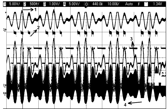
Figure 15. Oscilloscope waveforms of the envelope reference (label 1), multilevel's output voltage (label 2), envelope amplifier's output voltage (label 3) and the output of the implemented EER transmitter (label 4) when the reference signal is composed of two tones (200 kHz and 250 kHz)
