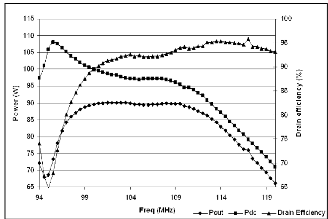
Figure 7. Measured output power and the efficiency of the implemented class E for different switching frequencies (instrument accuracy: 5%).
