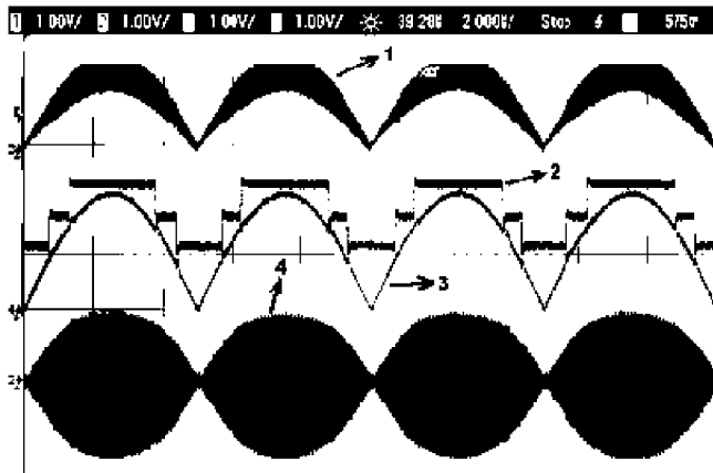
Figure 16. Oscilloscope waveforms of envelope reference (label 1), multilevel's output voltage (label 2), envelope amplifier's output (label 3) and the output of the implemented EER transmitter (label 4) when the transmitter's reference is a simple DSB-SC signal with carrier of 125 MHz and a 100 kHz sine wave as the modulated signal
