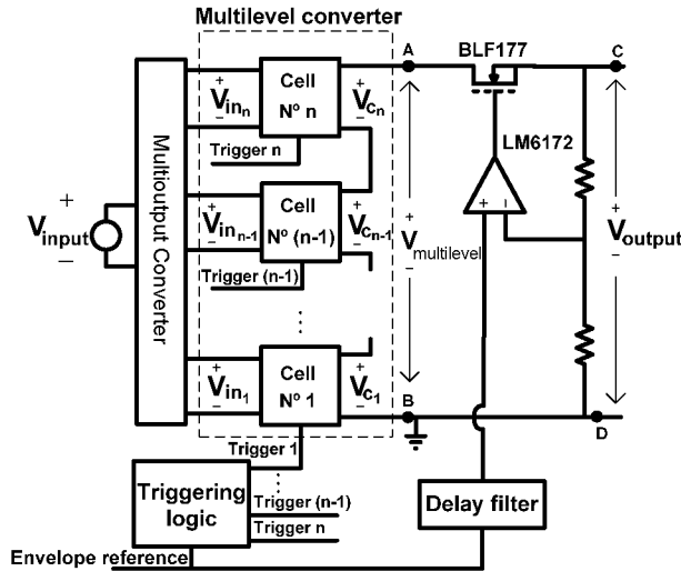
Figure 4. Simplified schematic of the implemented envelope amplifier
