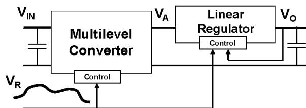
Figure 2. Simplified schematic of the proposed envelope amplifier
