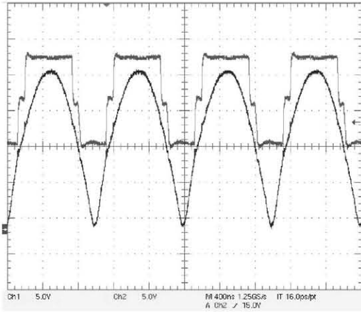
Figure 10. Waveform of multilevel's output voltage and linear regulator's output voltage when a rectified 500 kHz sine wave is used as the reference
