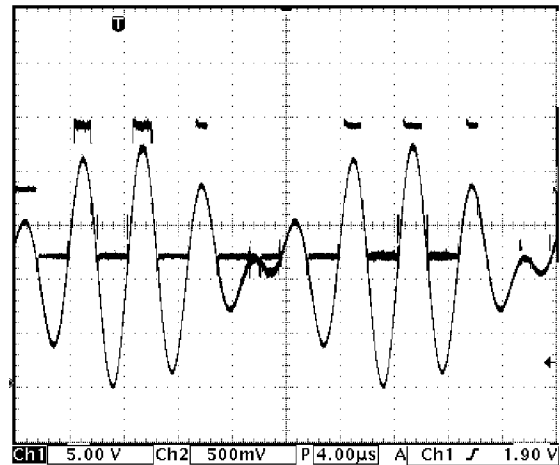
Figure 8. Output voltage of the multilevel converter and envelope amplifier when a two tone test is performed. Two tone signal consists of two sine waves of 200 kHz and 250kHz
