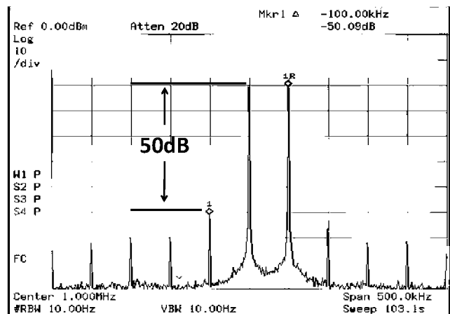
Figure 9. Attenuation of the intermodulation components measured by a spectral analyzer in the two tone test, when a sine waves of 1 MHz and 1.05 MHz are used.
