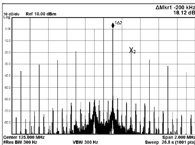
Figure 17. Spectrum of the transmitter's output signal when the system's reference is a simple DSB-SC signal with carrier of 125 MHz and a 100 kHz sine wave as the modulated signal
