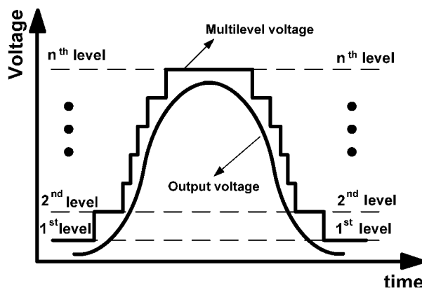
Figure 3. Time diagrams of the proposed envelope amplifier
