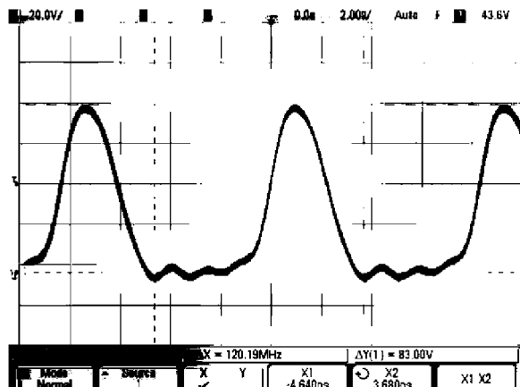
Figure 6. Drain voltage of the implemented class E amplifier when it operates at 120MHz
