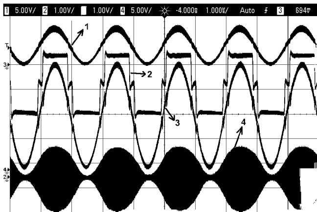
Figure 13. Oscilloscope waveforms of the envelope reference (label 1), multilevel's output voltage (label 2), envelope's amplifier output (label 3) and the EER transmitter's output (label 4), when the envelope reference is a 500 kHz sinewave
