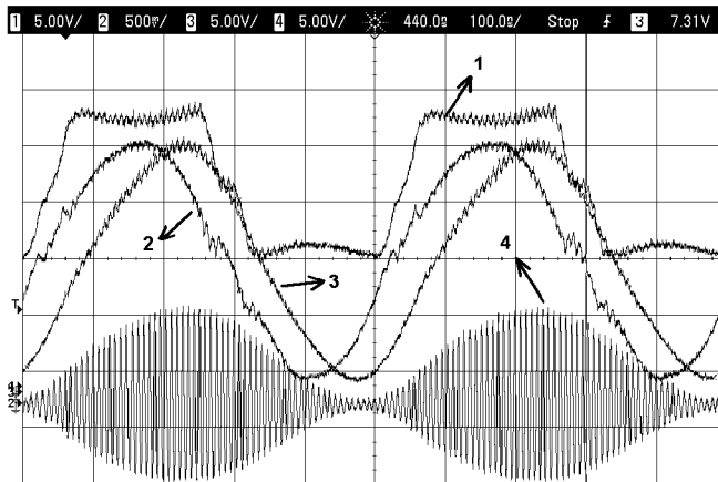
Figure 14. Oscilloscope waveforms of the multilevel's output (label 1), envelope amplifier's output (label 2), supply voltage of the class E amplifier (label 3) and the output of the implemented EER transmitter (label 4) when the envelope reference is a 2 MHz sine wave
