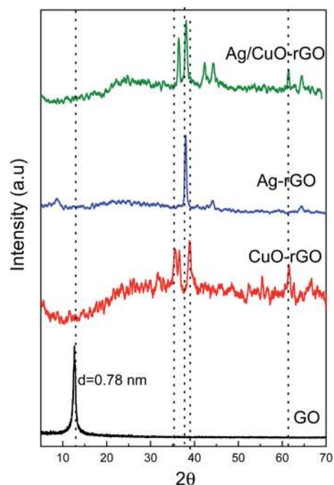
Fig. 2 XRD pattern of GO, CuO-rGO, Ag-rGO and Ag/CuO-rGO.
