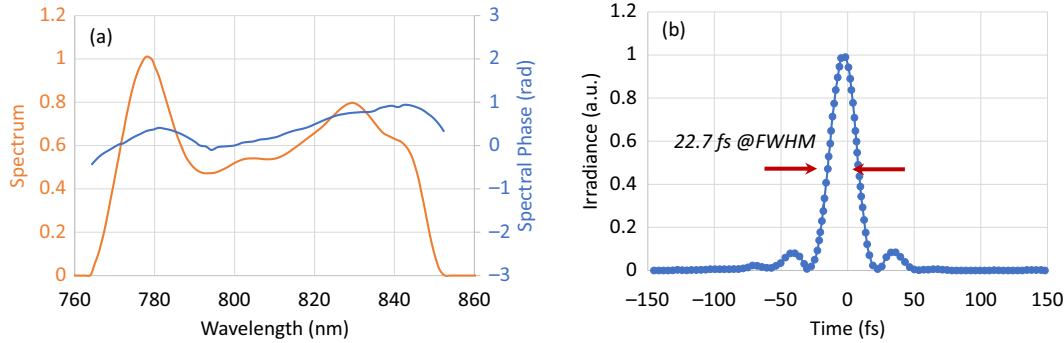
Figure 17. Wizzler measurements: (a) flat spectral phase and more than 70 nm spectral bandwidth; (b) reconstructed pulse with \tau = 22.7 FWHM duration.
