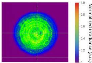
Figure 5. Near-field beam intensity profile of the 532 nm picosecond pump laser for OPCPA.
