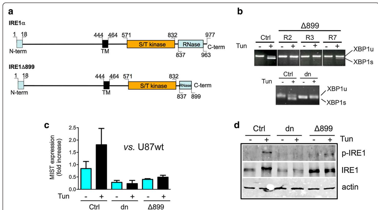
Figure 4 Characterization of U87 \Delta 899 IRE1 RNase dominant-negative cells. (a) The U87 \Delta 899 RNase construct was designed to express an IRE1 \alpha protein truncated at its cytoplasmic C-terminal end in the RNase domain. (b) Inhibition of XBP1 splicing in three different U87 \Delta 899 RNase clones (R2, R3 and R7, upper panel) and in U87dn cells (lower panel). Cells were stimulated for 2 h with 10 \mu g/ml tunicamycin/DMSO (Tun) or with DMSO only. Amplification of XBP1 transcripts was carried out after reverse transcription using primers flanking the XBP1 mRNA splicing sites. PCR products were analyzed by electrophoresis on 2% agarose gels. XBP1s and XBP1u represent spliced and unspliced mRNA, respectively. (c) MIST transcripts were measured by qPCR in U87wt, U87Ctrl, U87dn and U87 \Delta 899 cells subjected or not to tunicamycin treatment for 16 h. The reference value (1.00) corresponds to the value obtained with U87wt cells in the absence of tunicamycin. Results were normalized using HPRT1 mRNA as standard. qPCR was performed in triplicate on three independent RNA preparations. Data are presented as mean \pm SD. (d) IRE1 kinase autophosphorylation in U87 \Delta 899 cells. Immunoblotting analysis of total IRE1 \alpha (IRE1) and of phospho-Ser724-IRE1 (p-IRE1) proteins after a 2h-incubation with or without tunicamycin.
