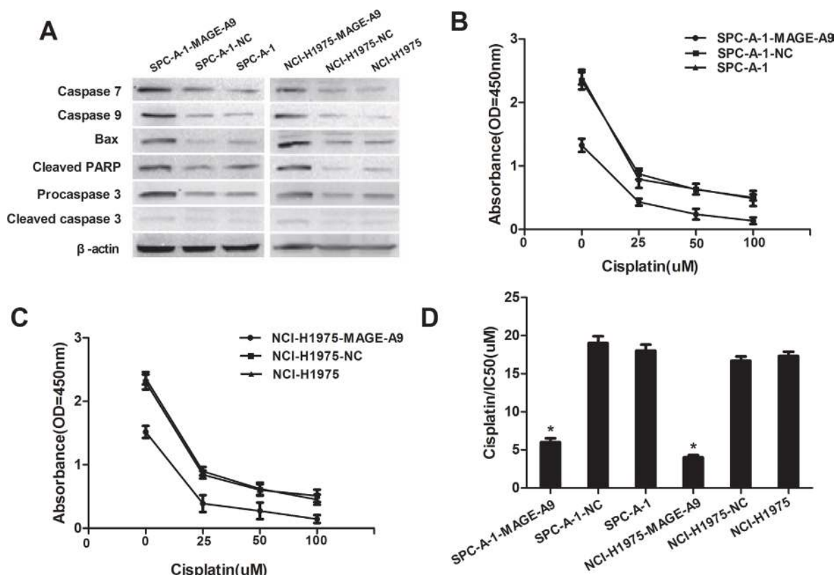
Figure 4: MAGE-A9 expression and apoptosis in vitro . (A) Western blot analysis of apoptosis-associated protein expression in MAGE-A9 silenced cells. \beta -Actin was used as a loading control. (B) and (C) MAGE-A9 depletion in SPC-A-1-MAGE-A9 and NCI-H1975-MAGE-A9 cells contributed to an increased apoptotic response to cisplatin. (Error bars = 95% confidence interval, CI; P < 0.05 ). (D) Half-maximal inhibitory concentration (IC 50 ) values of cisplatin. IC 50 values were determined using CCK-8 as described above. (Error bars = 95% CI; * P < 0.05 ).
