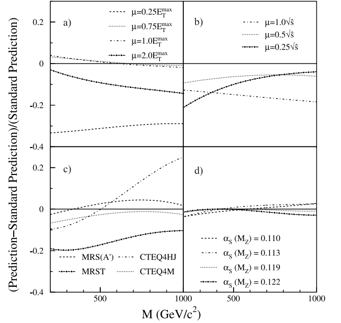
FIG. 12. The differences between the alternative predictions and the reference prediction ( \mu = 0.5E_T^{\text{max}} , CTEQ3M) of the inclusive dijet mass cross section [Eq. (4.15)] at \sqrt{s} = 1800 GeV for |\eta^{\text{j}i}| < 1.0 . Shown are the alternative predictions for the choices (a) \mu = (0.25, 0.75, 1.0, 2.0)E_T^{\text{max}} , (b) \mu = (0.25, 0.5, 1.0)\sqrt{s} and 0.5E_T^{\text{j}1} , (c) CTEQ4M, CTEQ4HJ, MRS(A'), and MRST, and (d) for \alpha_s = 0.110 - 0.122 using the CTEQ4A PDFs compared with the calculation using CTEQ4M, for which \alpha_s = 0.116 .
