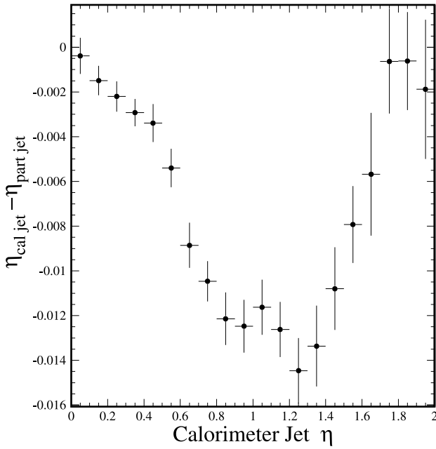
FIG. 7. HERWIG Monte Carlo simulation of the \eta bias for all jet energies as a function of the reconstructed jet \eta .
