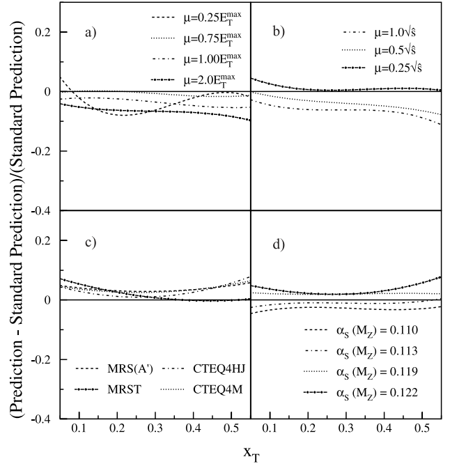
FIG. 10. The difference between alternative predictions and the reference prediction ( \mu = 0.5E_T^{\text{max}} , CTEQ3M) of the ratio of inclusive jet cross sections at \sqrt{s} = 630 and 1800 GeV for |\eta^{\text{jet}}| < 0.5 . Shown are the alternative predictions for the choices (a) \mu = (0.25, 0.75, 1.0, 2.0)E_T^{\text{max}} , (b) \mu = (0.25, 0.5, 1.0)\sqrt{s} and 0.5E_T^{\text{jet}} , (c) CTEQ4M, CTEQ4HJ, MRS(A'), and MRST, and (d) for \alpha_s = 0.110 - 0.122 using the CTEQ4A PDFs compared with the calculation using CTEQ4M, for which \alpha_s = 0.116 .
