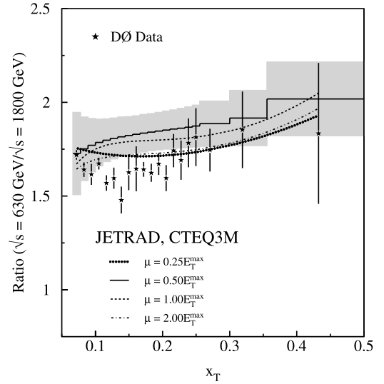
FIG. 67. The ratio of dimensionless cross sections for |\eta| < 0.5 compared with JETRAD predictions with various values of \mu and the CTEQ3M PDF. The shaded band represents the \pm 1\sigma systematic uncertainty band about the prediction.
