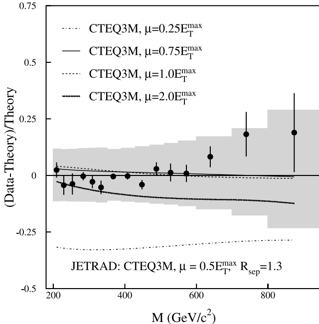
FIG. 94. The difference between the data and the prediction (JETRAD) divided by the prediction for |\eta^{\text{jel}}| < 1.0 . The solid circles represent the comparison to the calculation using CTEQ3M with \mu = 0.5E_T^{\text{max}} . The shaded region represents the \pm 1\sigma systematic uncertainties about the prediction. The effects of changing the renormalization scale are also shown (each curve shows the difference between the alternative prediction and the prediction using CTEQ3M with \mu = 0.5E_T^{\text{max}} ).
