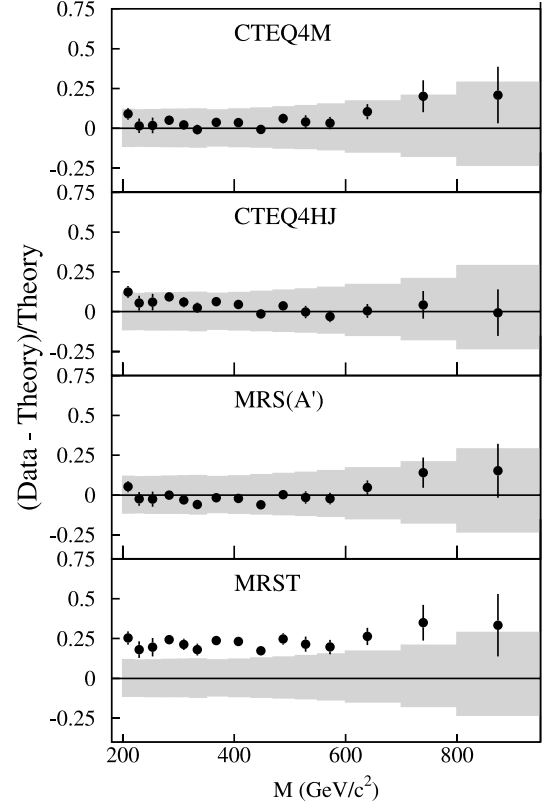
FIG. 95. The difference between the data and the prediction (JETRAD) divided by the prediction for |\eta^{\text{jel}}| < 1.0 . The solid circles represent the comparison to the calculation using \mu = 0.5E_T^{\text{max}} and the PDFs CTEQ4M, CTEQ4HJ, MRS(A'), and MRST. The shaded region represents the \pm 1\sigma systematic uncertainties about the prediction.
