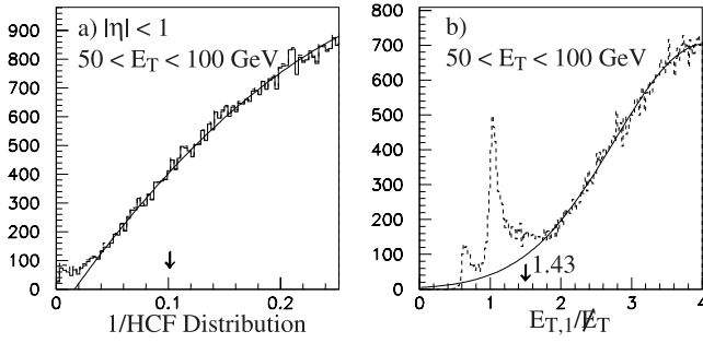
FIG. 16. (a) The 1/\text{HCF} distribution. The arrow shows the location of the cut for \sqrt{s}=1800 GeV. (b) The distribution of E_T^{\text{jet1}}/E_T . The arrow at E_T^{\text{jet1}}/E_T=1.43 corresponds to the E_T/E_T^{\text{jet1}} cut of 0.7. The peak at 1.0 is due to contamination from cosmic rays and the main ring. The dashed histograms show the distributions for the full data samples.
