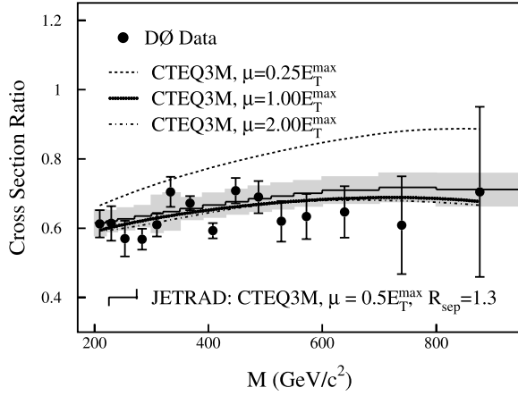
FIG. 93. The ratio of cross sections for |\eta^{\text{jel}}| < 0.5 and 0.5 < |\eta^{\text{jel}}| < 1.0 for data (solid circles) and theory (various lines). The error bars show the statistical uncertainties. The shaded region represents the \pm 1\sigma systematic uncertainties about the prediction. The effects on the prediction of changing the renormalization scale are also shown.
