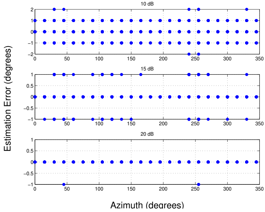
Figure B.4: f_c = 11 MHz Error Distribution vs. Azimuth for multiple SNR values using N_A = 16 individual feed points.
